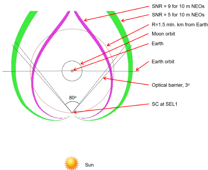
Figure 2. Detection zones of 10 m bodies.
