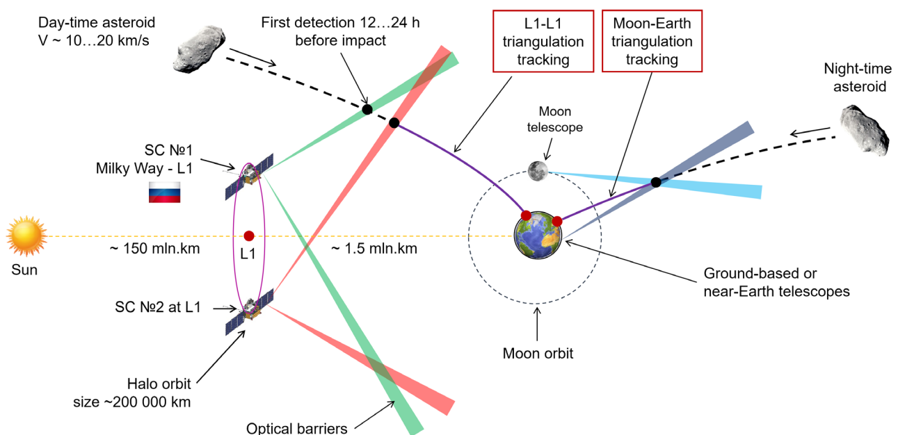
Figure 1. Scheme of operation for two SODA SC option which enables triangulation mode.
